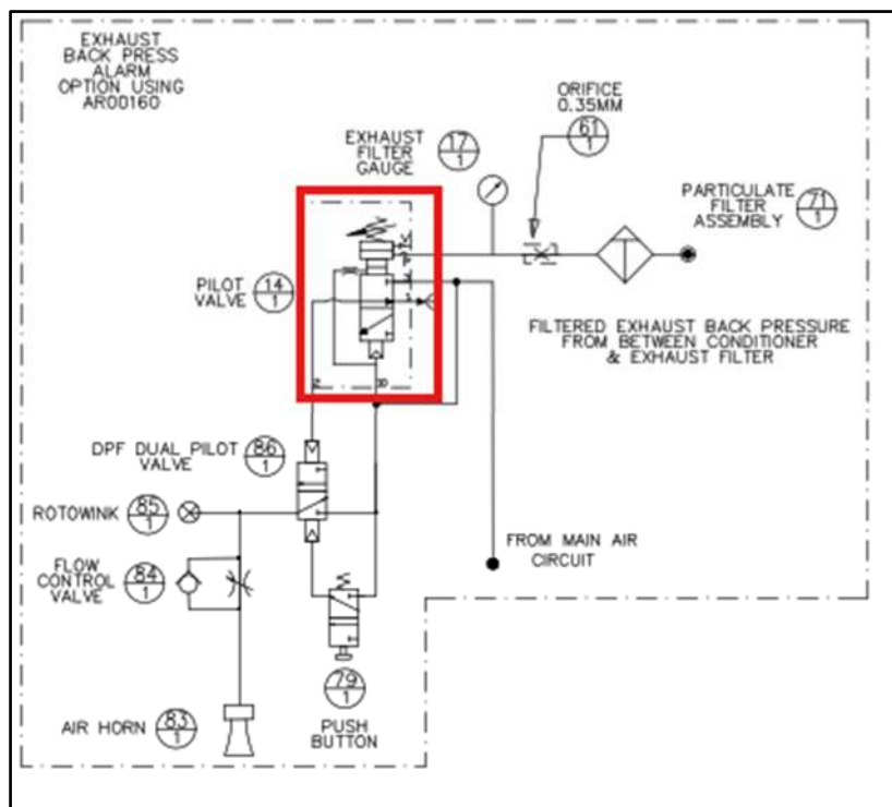
Figure 5: AR00160 hosing when connected as a DPF alarm valve
