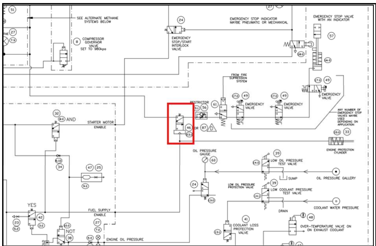
Figure 3: Strangler pilot valve replacement location on schematic – refer 7-161835-700
