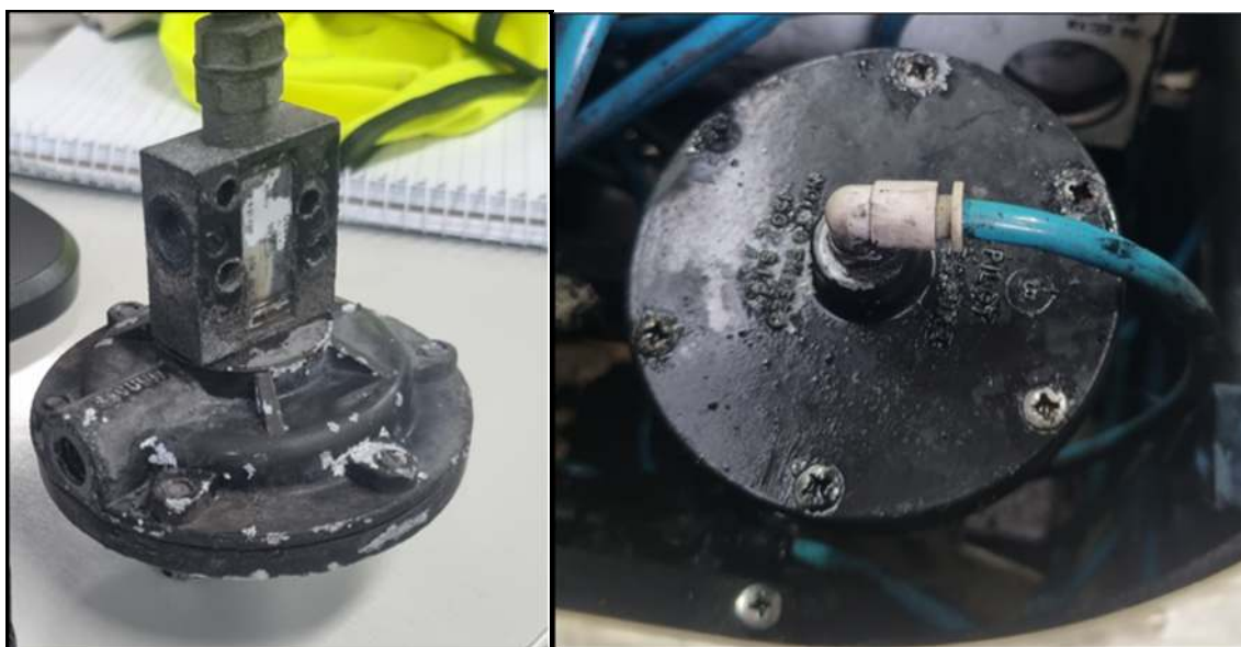
Figure 1a & 1b: original obsolete valve 7-182208-805
