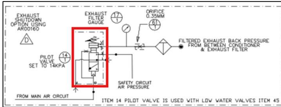
Figure 6: AR00160 hosing when connected as a DPF backpressure shutdown valve
