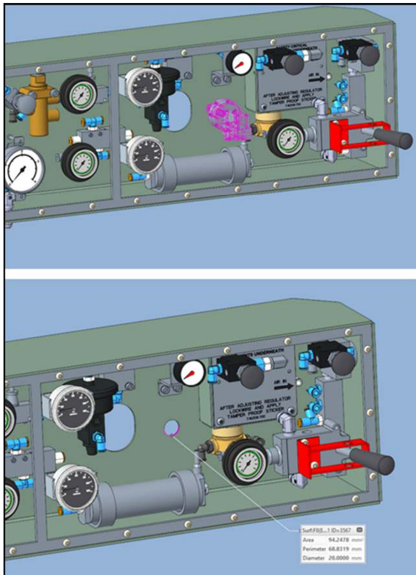
Figures 7a & b: Mounting information for AR00160
