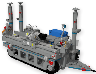
LMC 110T TRACK MOUNTED DRILL RIG
