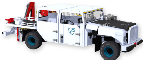
MK8 MINECRUISER AVAILABLE IN TROOP AND UTE VARIANTS MID AND HIGH SEAM VARIANTS
