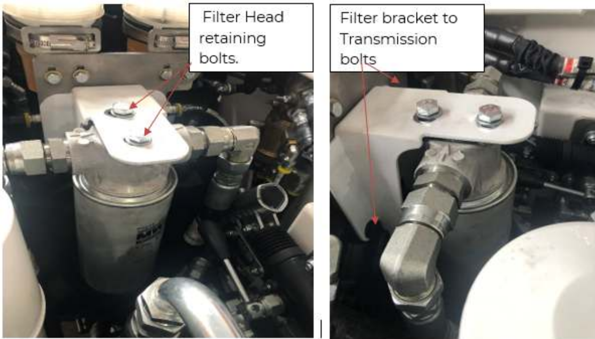
Remote oil filter bracket – fastener locations
